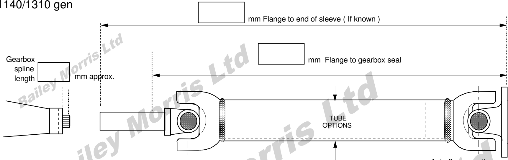
Gearbox Sleeve
